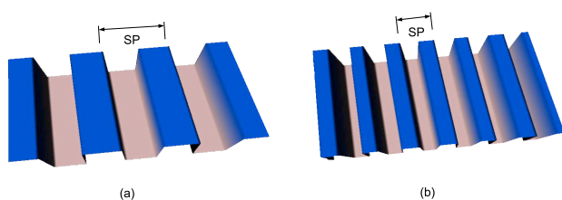
Figure 5: Examples of virtual textured surface that can be simulated on the tactile display. In this case, blue areas are the one with the greater friction coefficient. The spatial period (SP) in (a) is larger than in (b).
