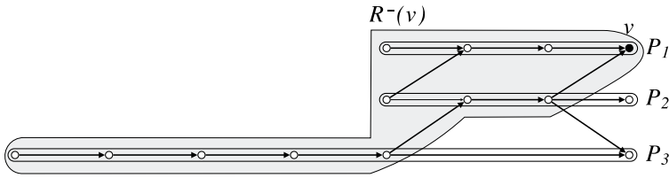
Fig. 2. A path cover P_1, P_2, P_3 of a DAG. We mark in gray the set R^-(v) of nodes that reach v .
